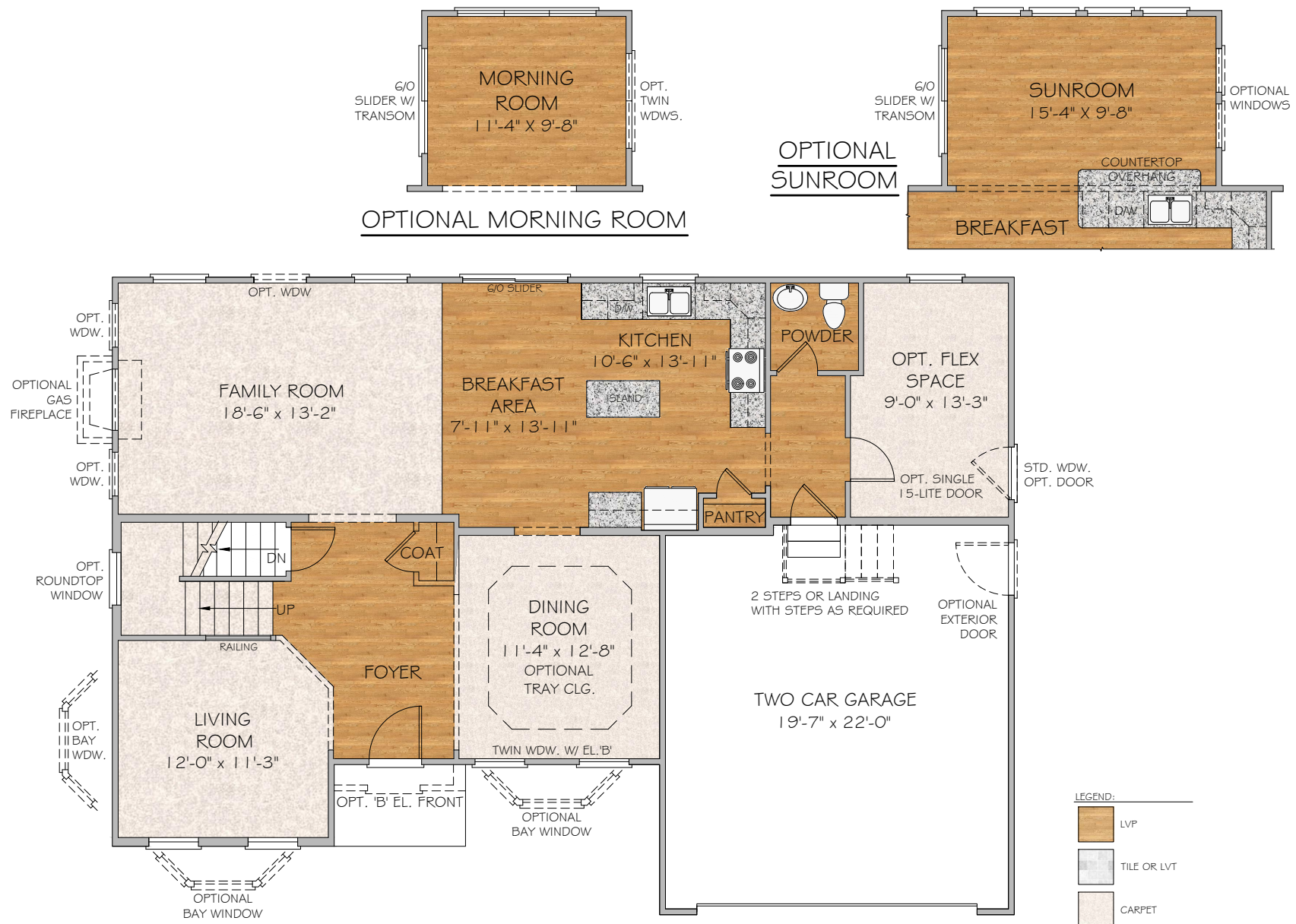
FIRST FLOOR PLAN WITH OPTIONAL FLEX SPACE
