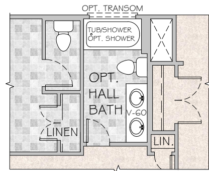
OPTIONAL HALL BATH LAYOUT
